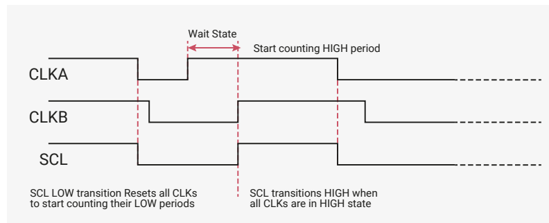
Figure 86. Multi-Master Clock Synchronisation
