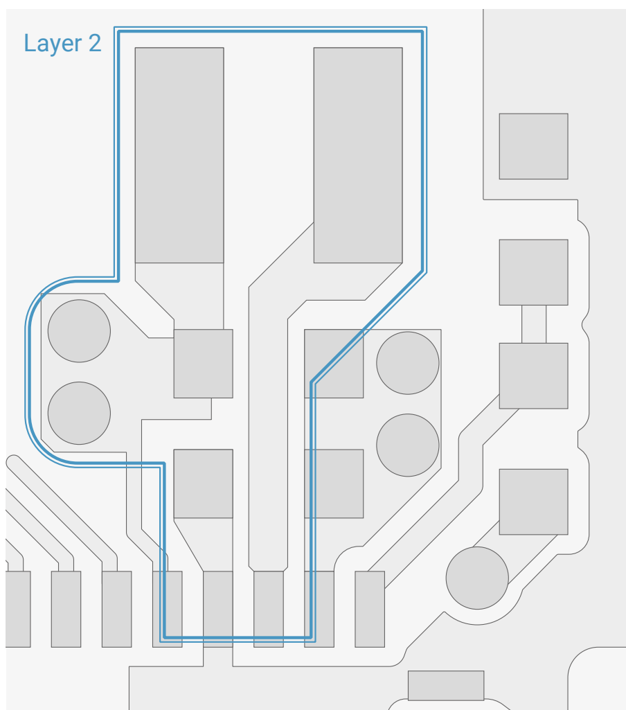
Figure 24. Cut-out beneath L_X/VREG\_LX net on layer 2 of 4 (or more) layer PCBs
